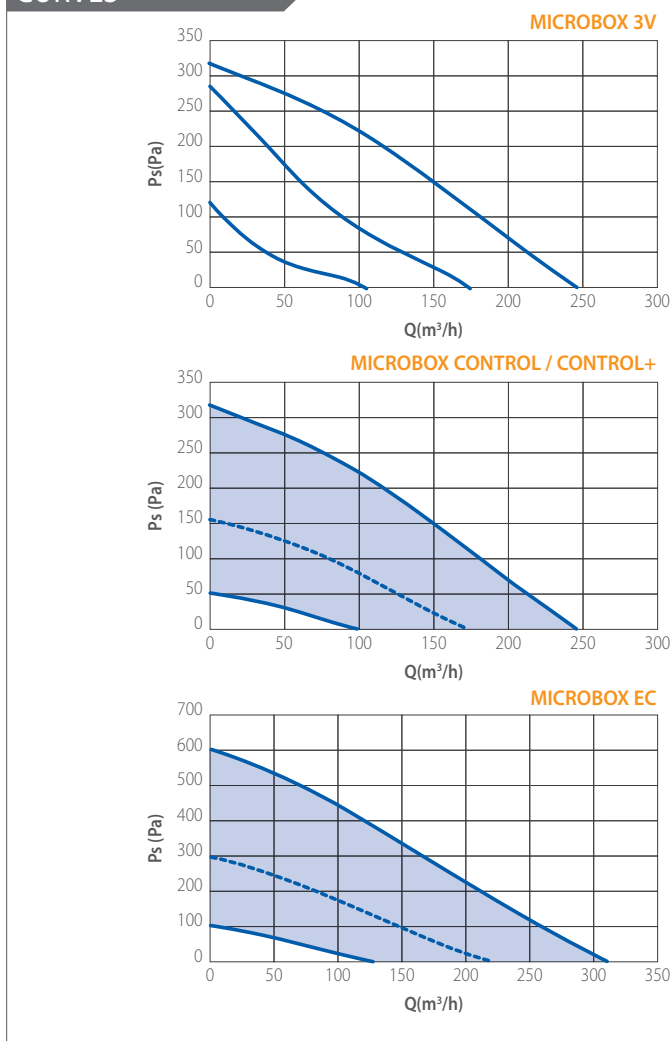
CP Suitable for Microbox Control See pag. 79
