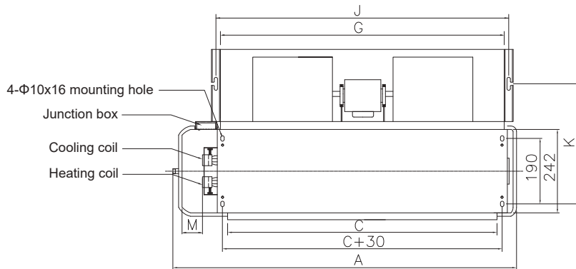
Side view of the unit without an air return plenum
