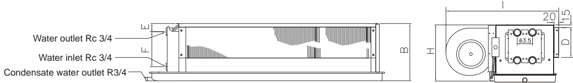
Side view of the unit without an air return plenum
